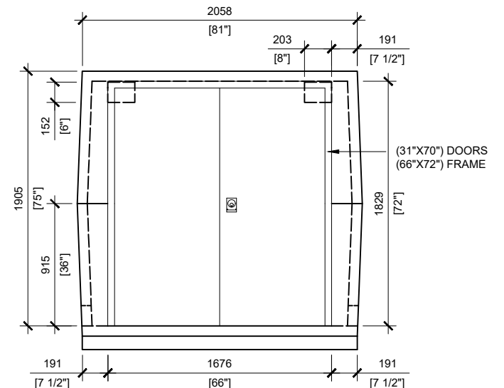
LEFT VIEW SCALE: 1/40
