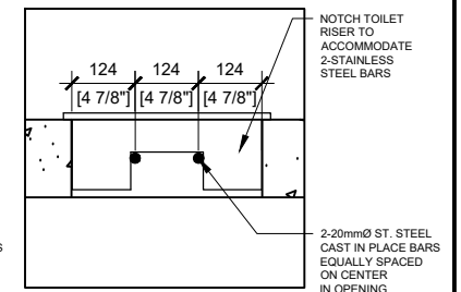
DETAIL 2: TOILET UNIT SECTION SCALE: 1/16
