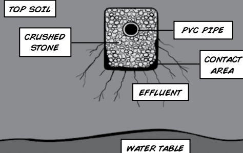
CONVENTIONAL SEPTIC BED
