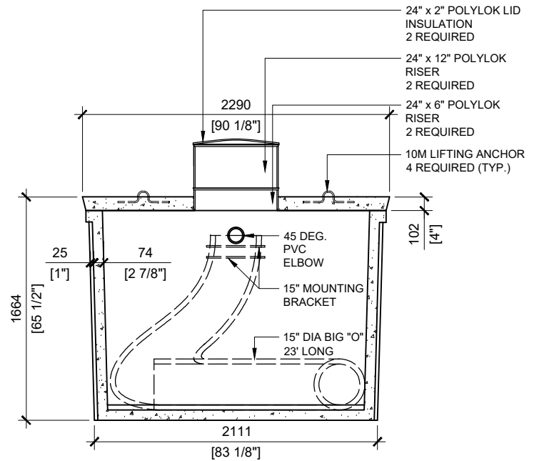
SECTION B SCALE:1/40
