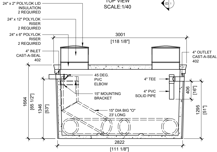
SECTION A SCALE:1/40
