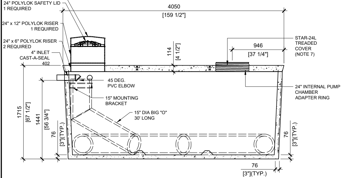
SECTION A SCALE:1/40
