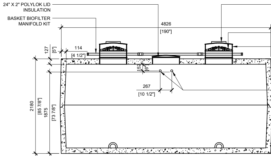
SECTION A SCALE:1/50
