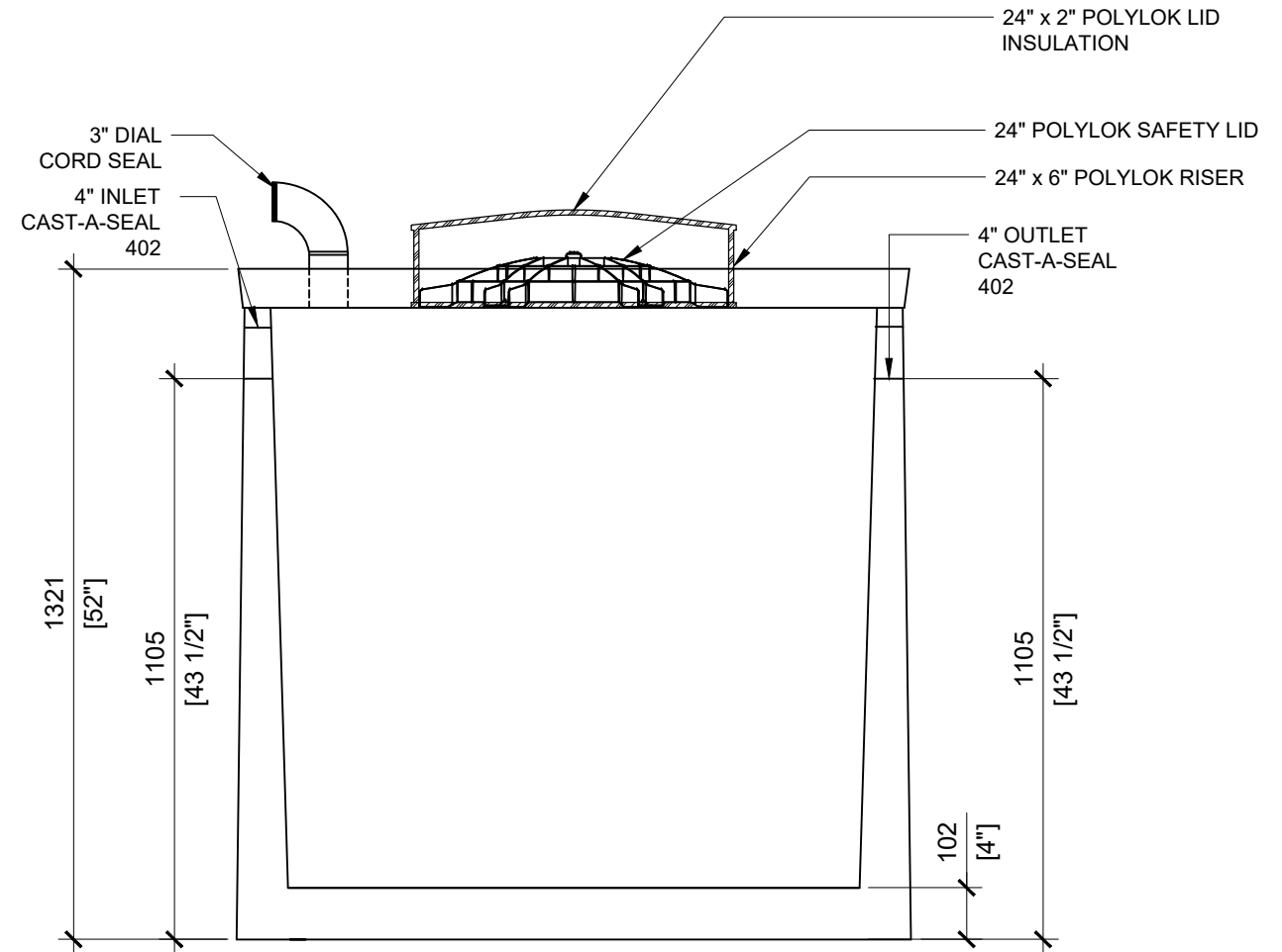
FRONT VIEW SCALE: 1/20
