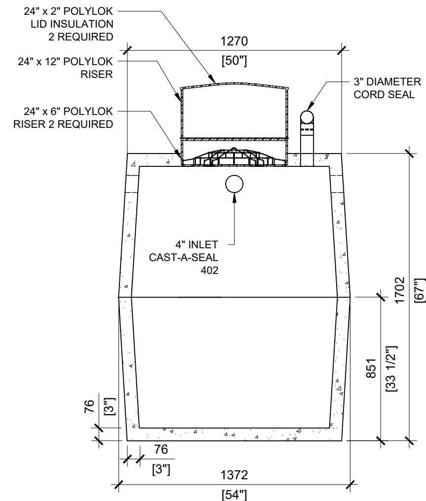
SECTION B SCALE:1/30
