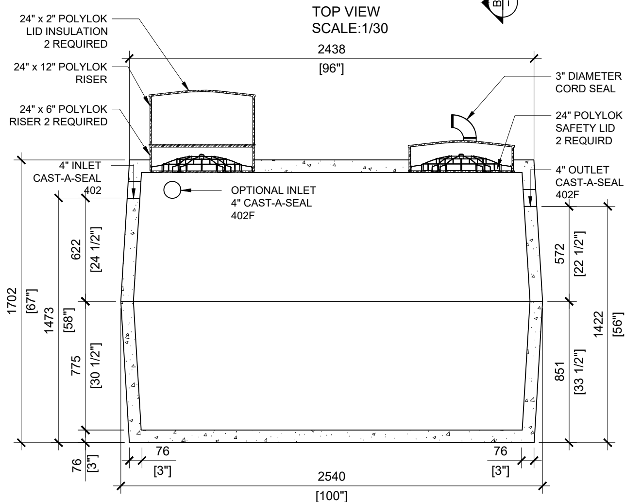
SECTION A SCALE:1/30
