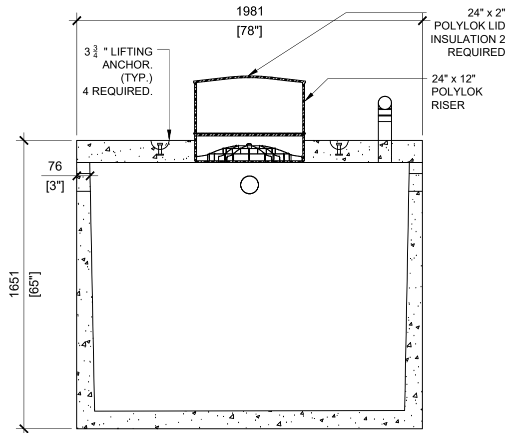
SECTION B SCALE:1/30
