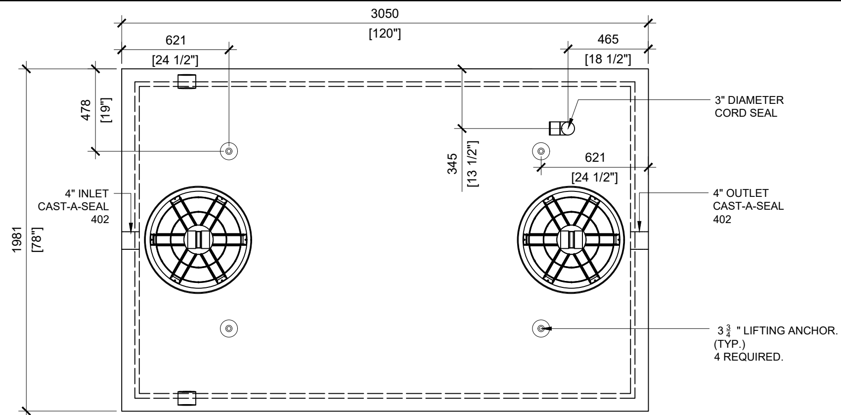
TOP VIEW SCALE:1/30
