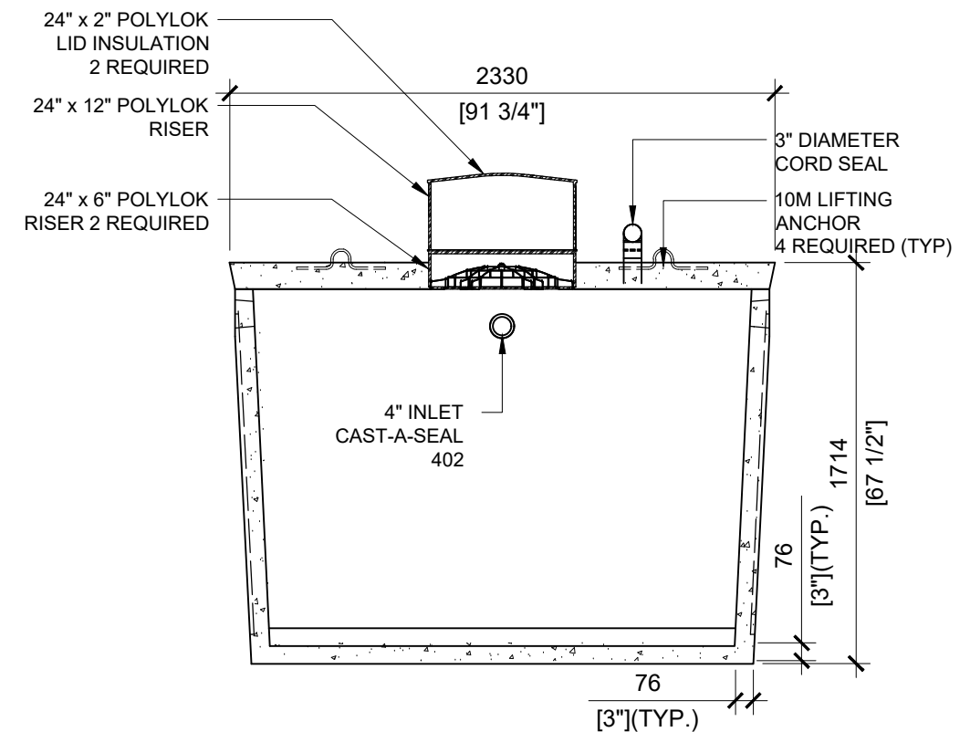
SECTION B SCALE:1/40
