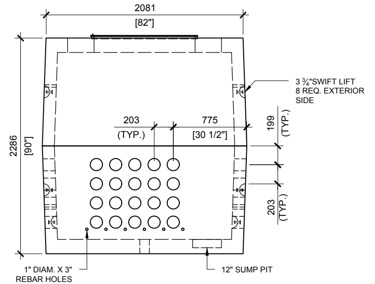
RIGHT VIEW SCALE: 1/40
