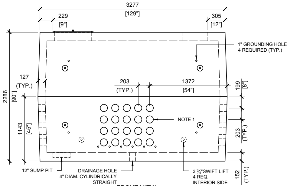
FRONT VIEW SCALE: 1/40
