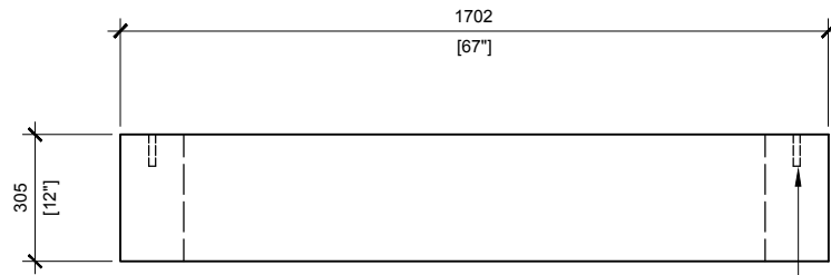
FRONT VIEW SCALE: 1/40
