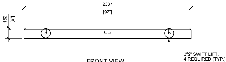
FRONT VIEW SCALE:1/30
