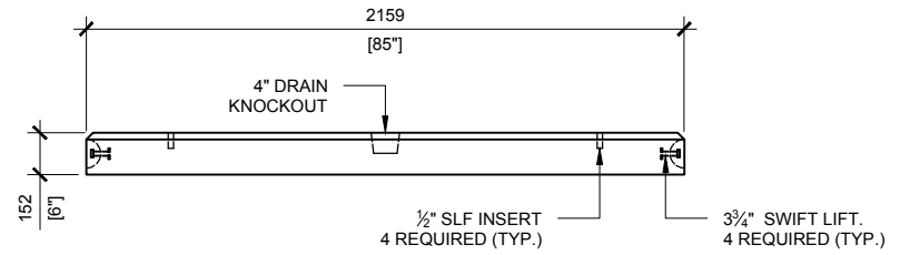
RIGHT VIEW SCALE:1/30
